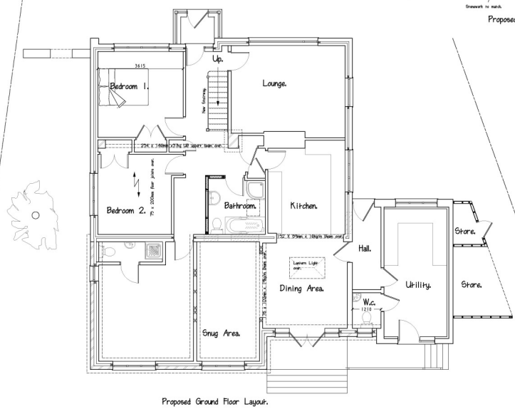
Proposed Ground Floor Layout.
